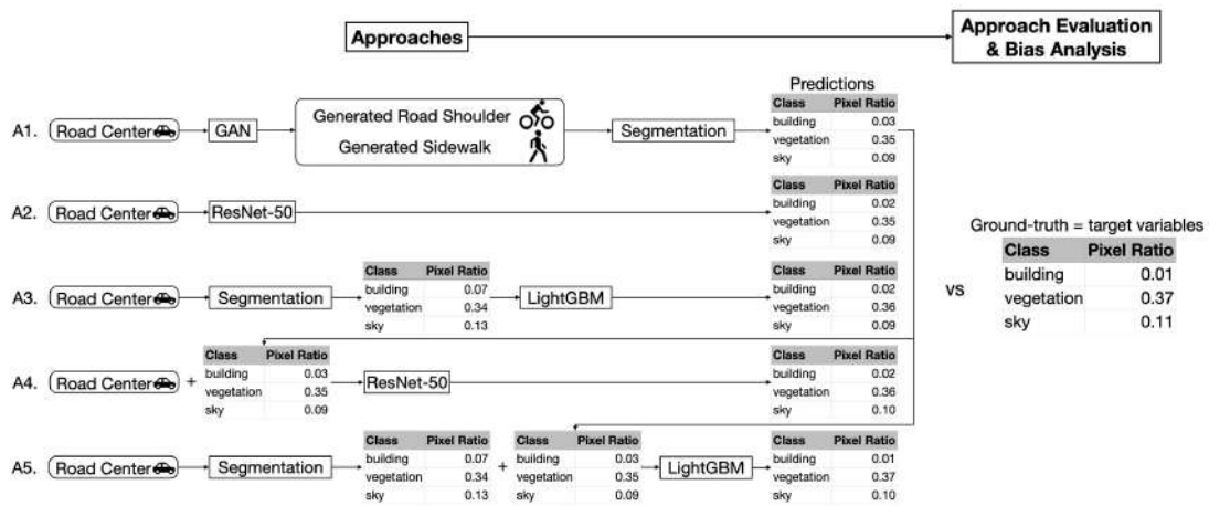
Figure 4.: This figure shows five approaches (i.e., A1-A5) used in this study and their evaluation. A1 generates road shoulder/sidewalk SVI using GAN models (i.e., Pix2Pix and CycleGAN) and obtains target pixel ratios through segmentation. A2 employs ResNet-50 to predict the target pixel ratios. A3 utilizes LightGBM with road center SVI pixel ratios as input to forecast the target pixel ratios. A4 inputs both road center SVI and pixel ratios from the GAN output into ResNet-50 to predict the target pixel ratios. A5 uses LightGBM with pixel ratios from both the road center SVI and the GAN output to predict the target pixel ratios.
